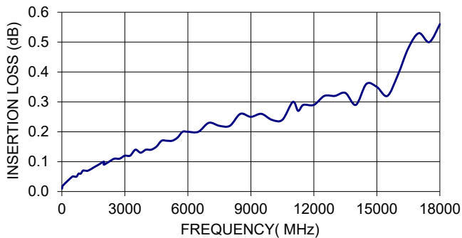
141-6SM+ INSERTION LOSS
