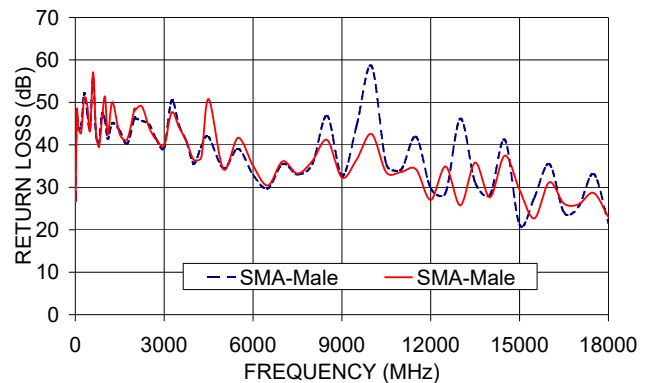
141-14SM+ RETURN LOSS
