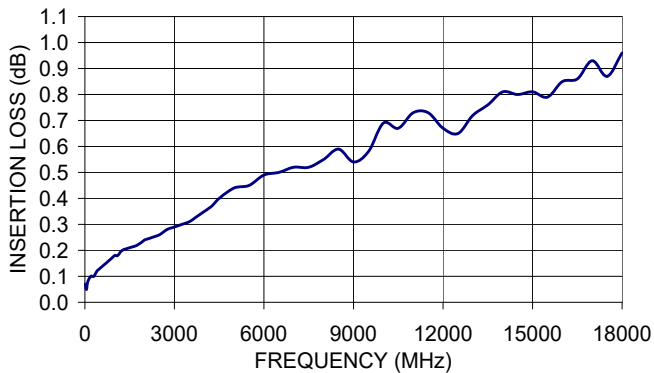
141-14SM+ INSERTION LOSS
