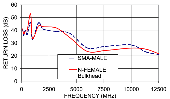
141-12SMNB+ RETURN LOSS
