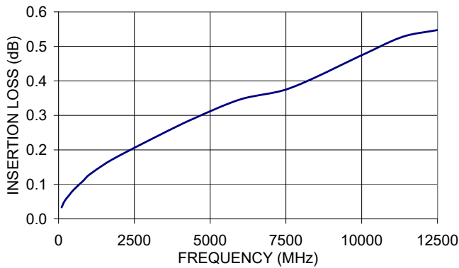
141-12SMNB+ INSERTION LOSS
