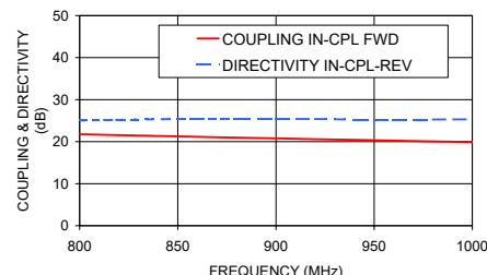
SYBD-20-13HP+ COUPLING & DIRECTIVITY
