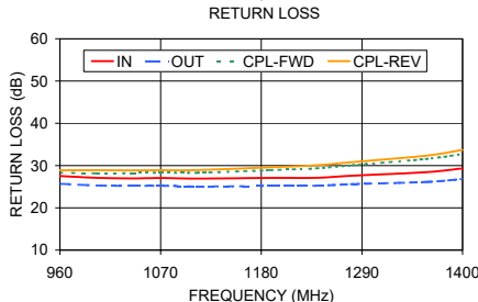
SYBD-18-142HP+ RETURN LOSS
