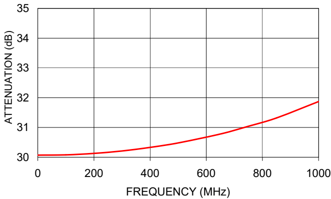
LAT-30+ ATTENUATION
