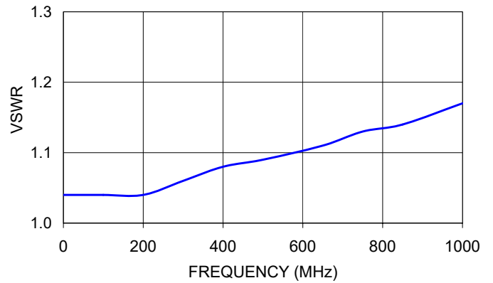
LAT-30+ VSWR
